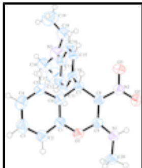
Fig. 1. : The molecular structure of (I), showing displacement ellipsoids drawn at the 50% probability level.
